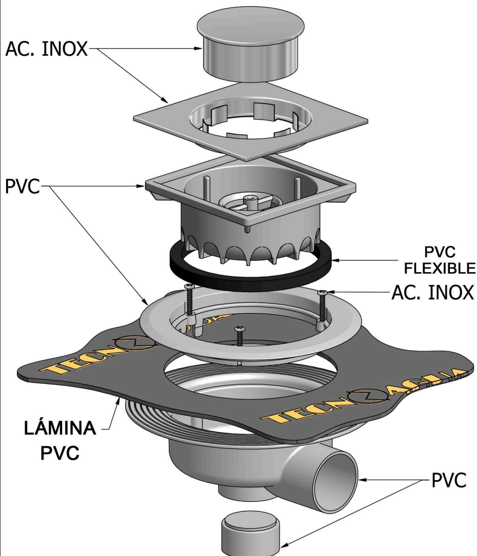
DESPIECE
