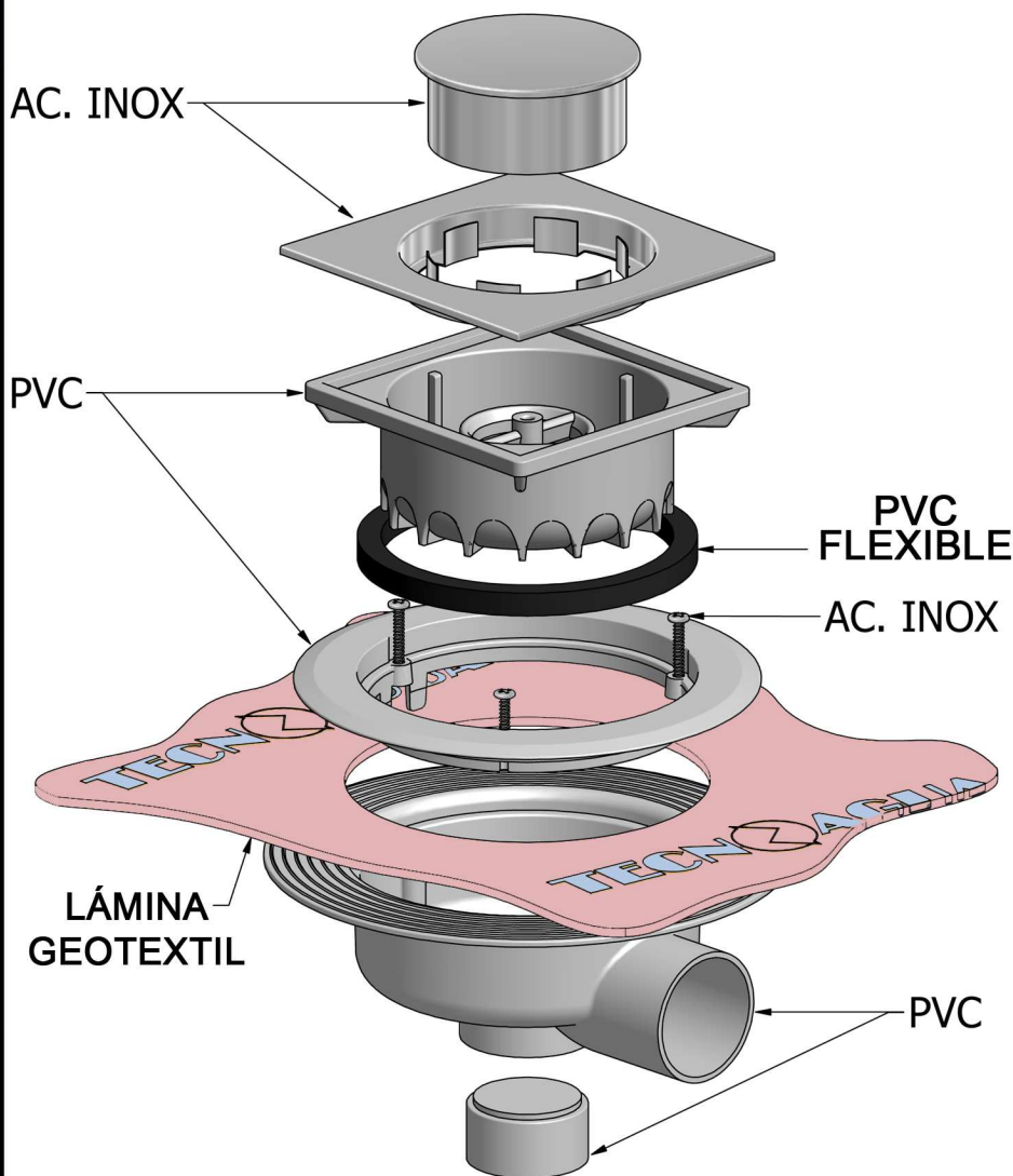
DESPIECE
