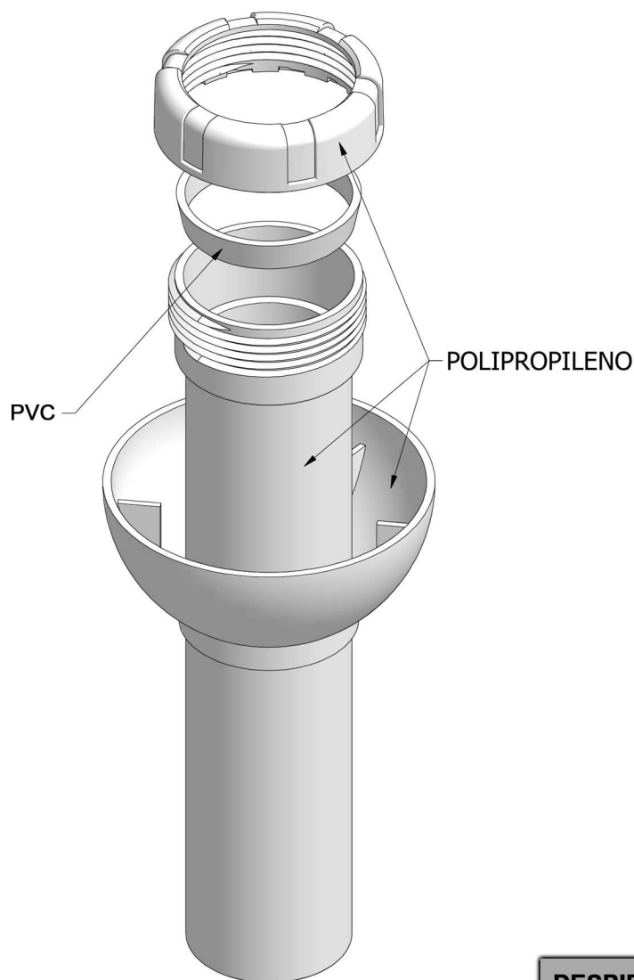
DESPIECE
