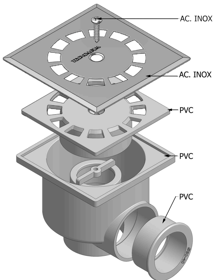
DESPIECE
