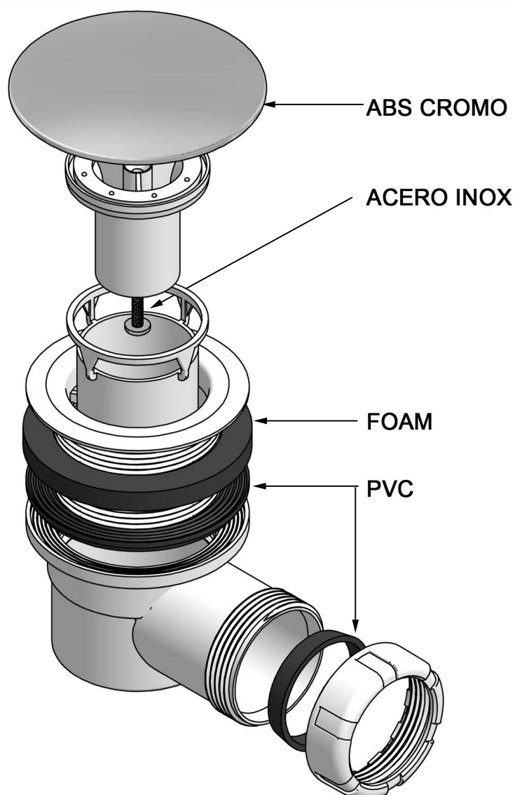
DESPIECE
